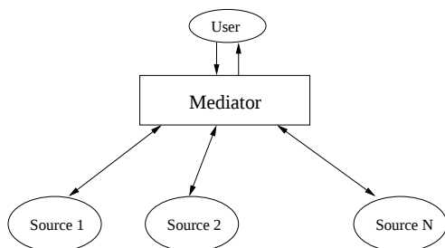
Figure 1: The TSIMMIS Architecture
